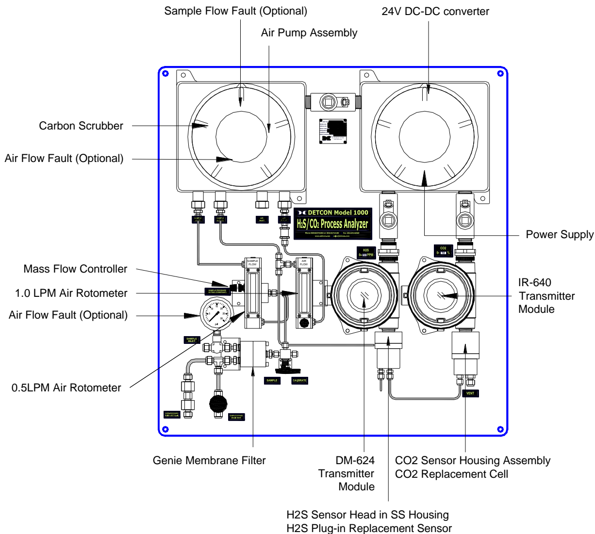
Figure 28 Analyzer with Air Dilution Spare Parts
