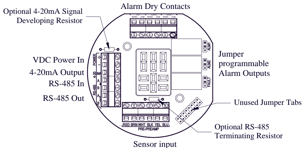
Figure 12 Connector Board Terminals
