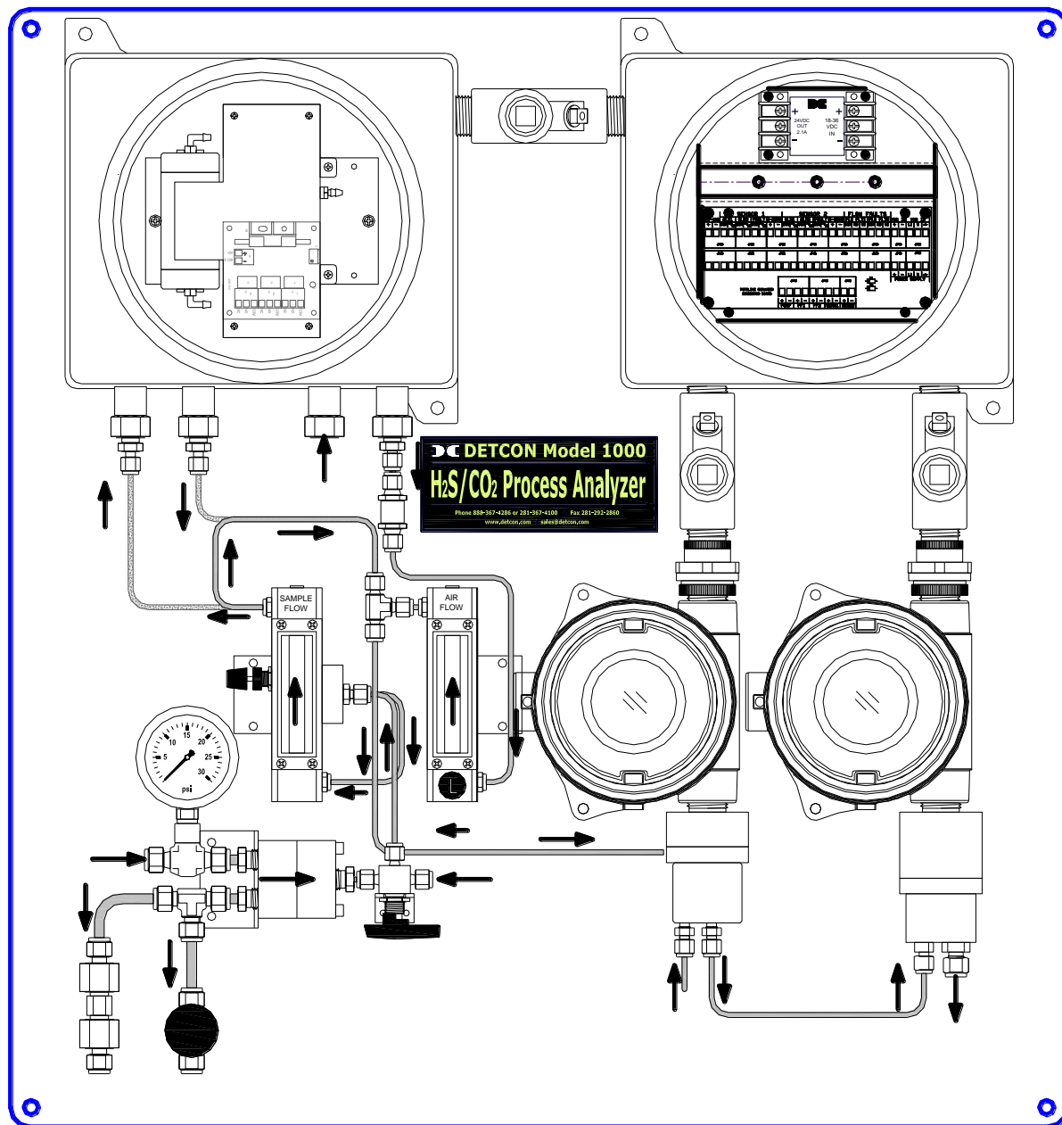
Figure 30 Unit Flow Diagram with dilution
