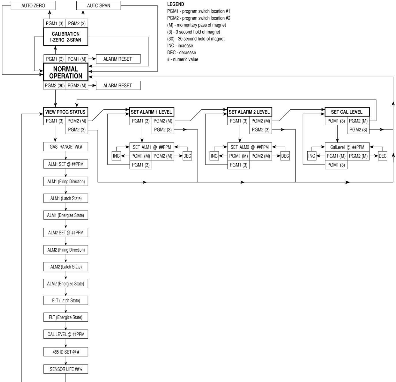
Figure 23 DM-624 Software Flow Chart
