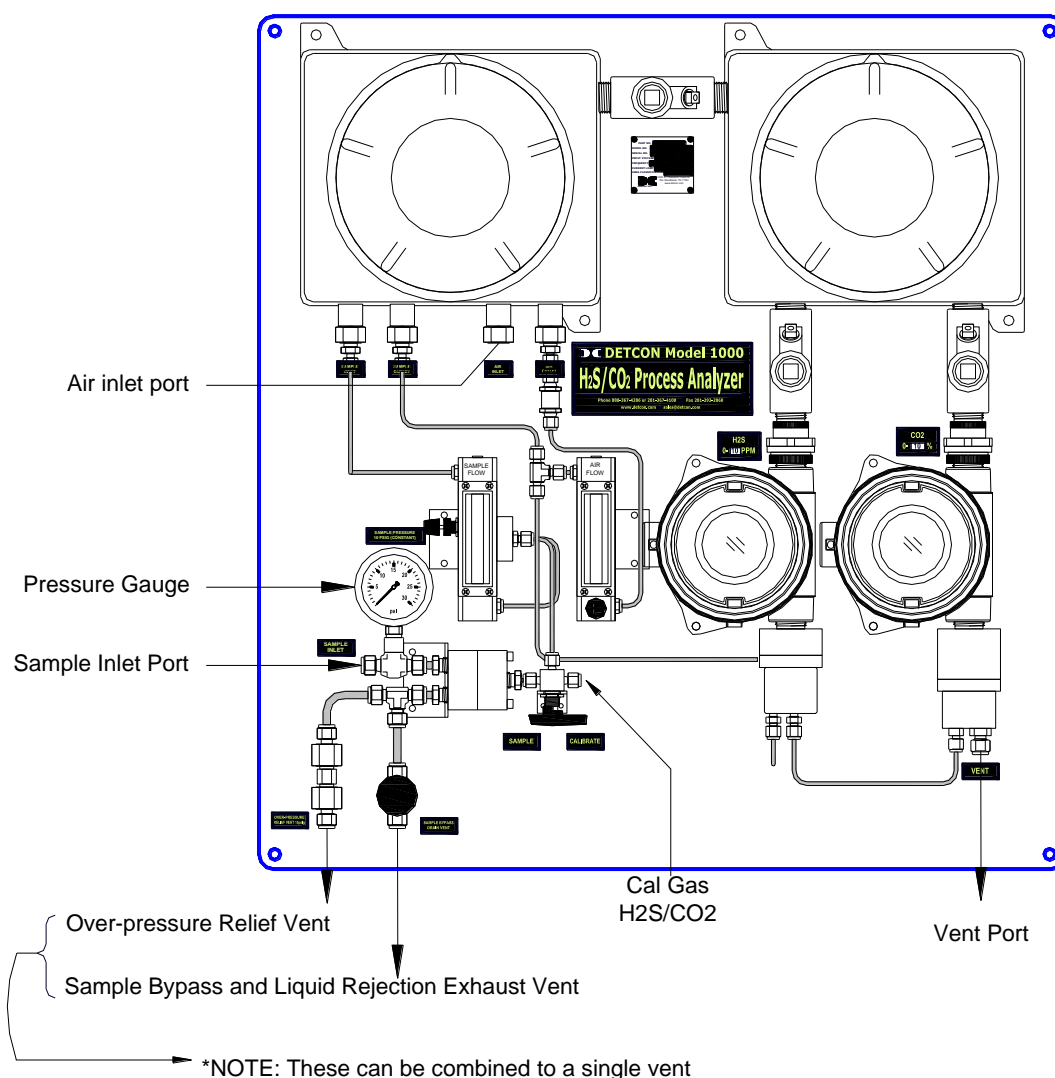
Figure 16 Port Identification with Dilution
