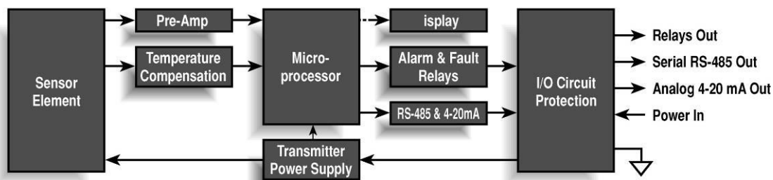
Figure 10 Functional Block Diagram
