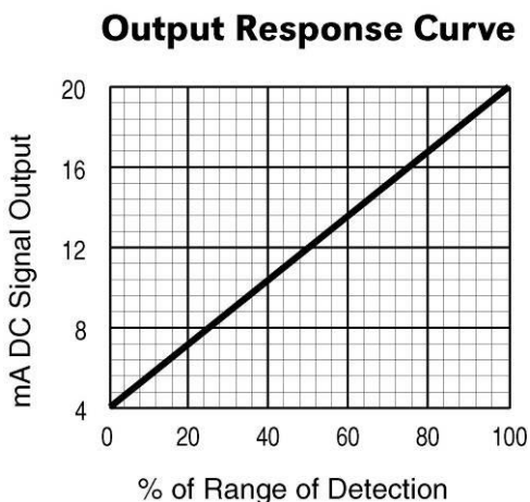
Figure 8 Response Curve
