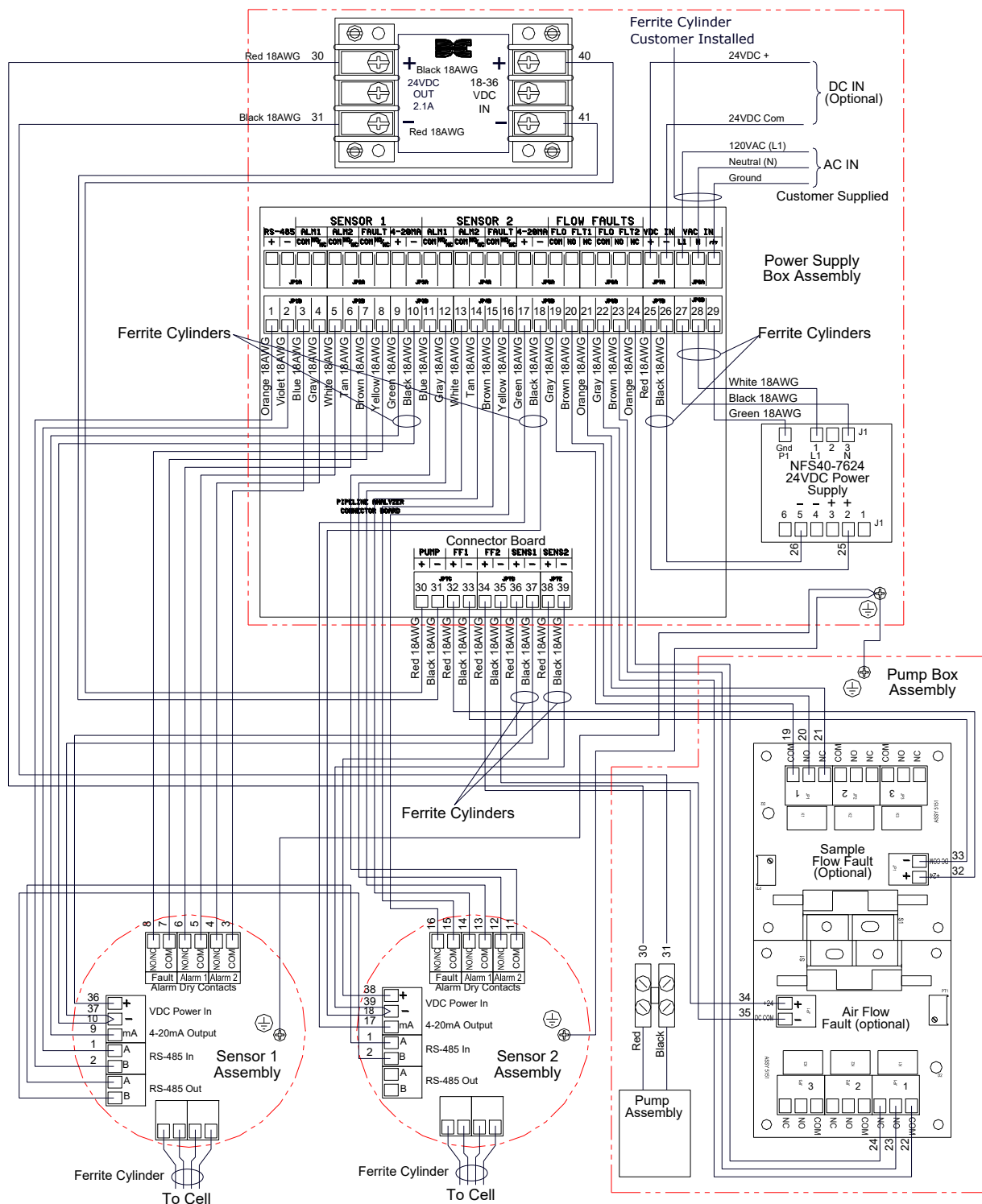
Figure 32 Wiring Diagram
