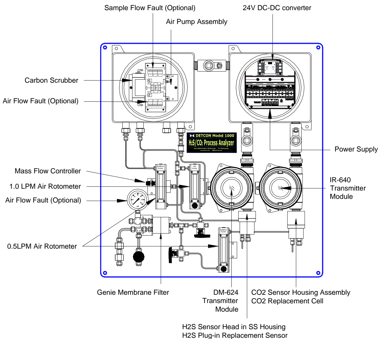
Figure 27 Analyzer Spare Parts
