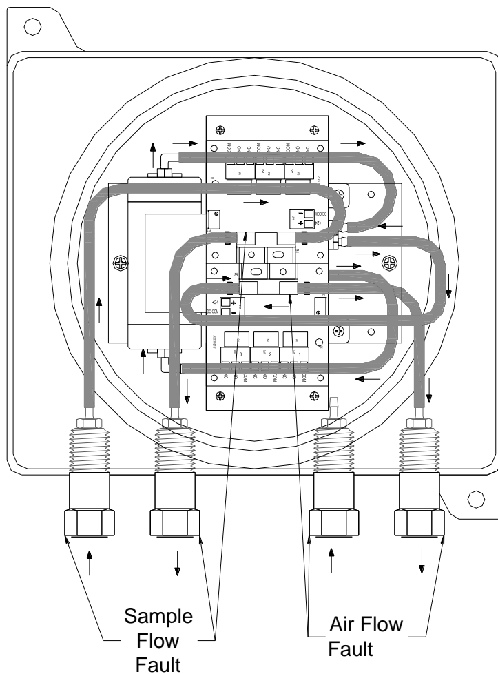
Figure 31 Pump Box Flow Diagram
