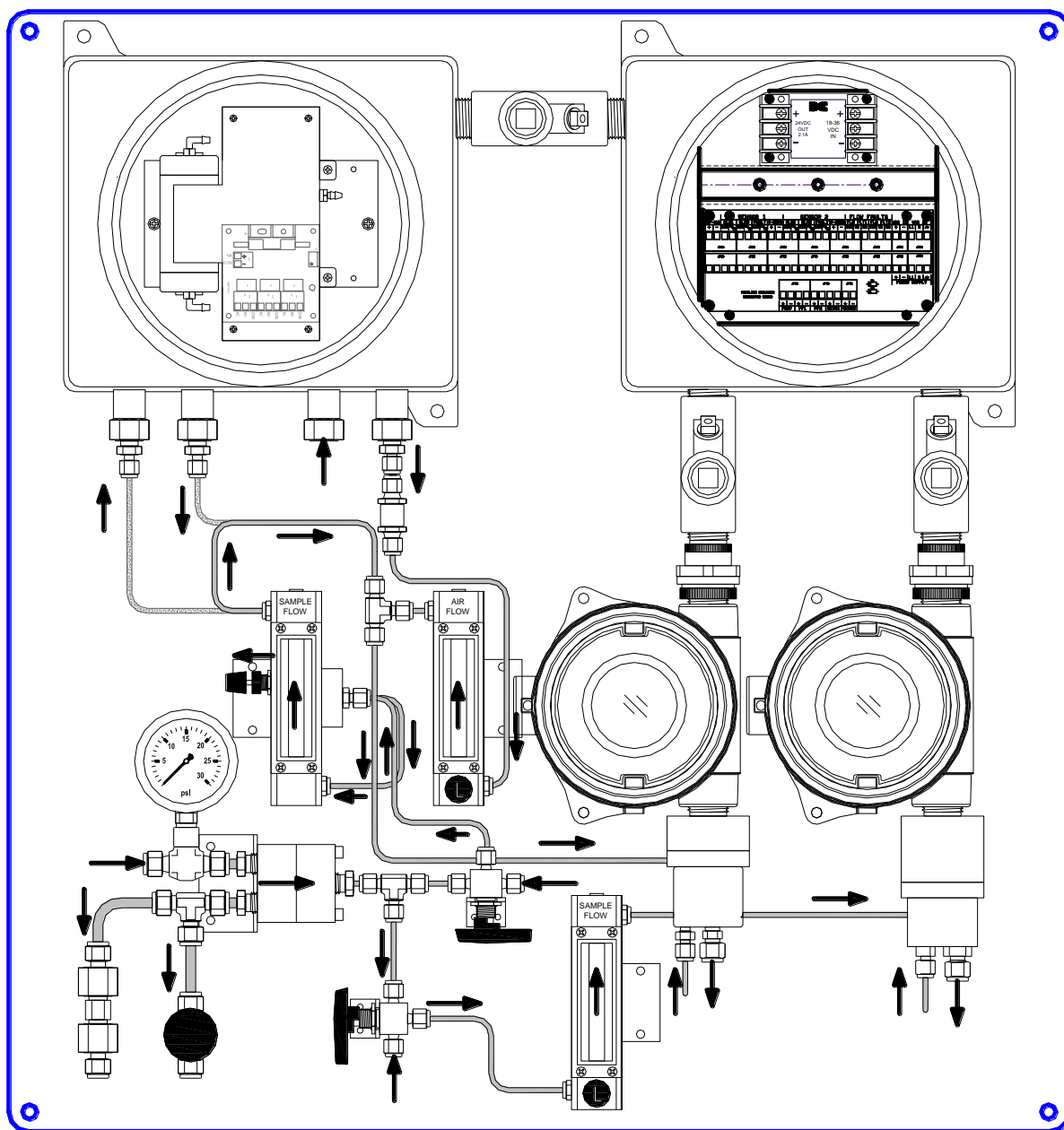
Figure 29 Unit Flow Diagram
