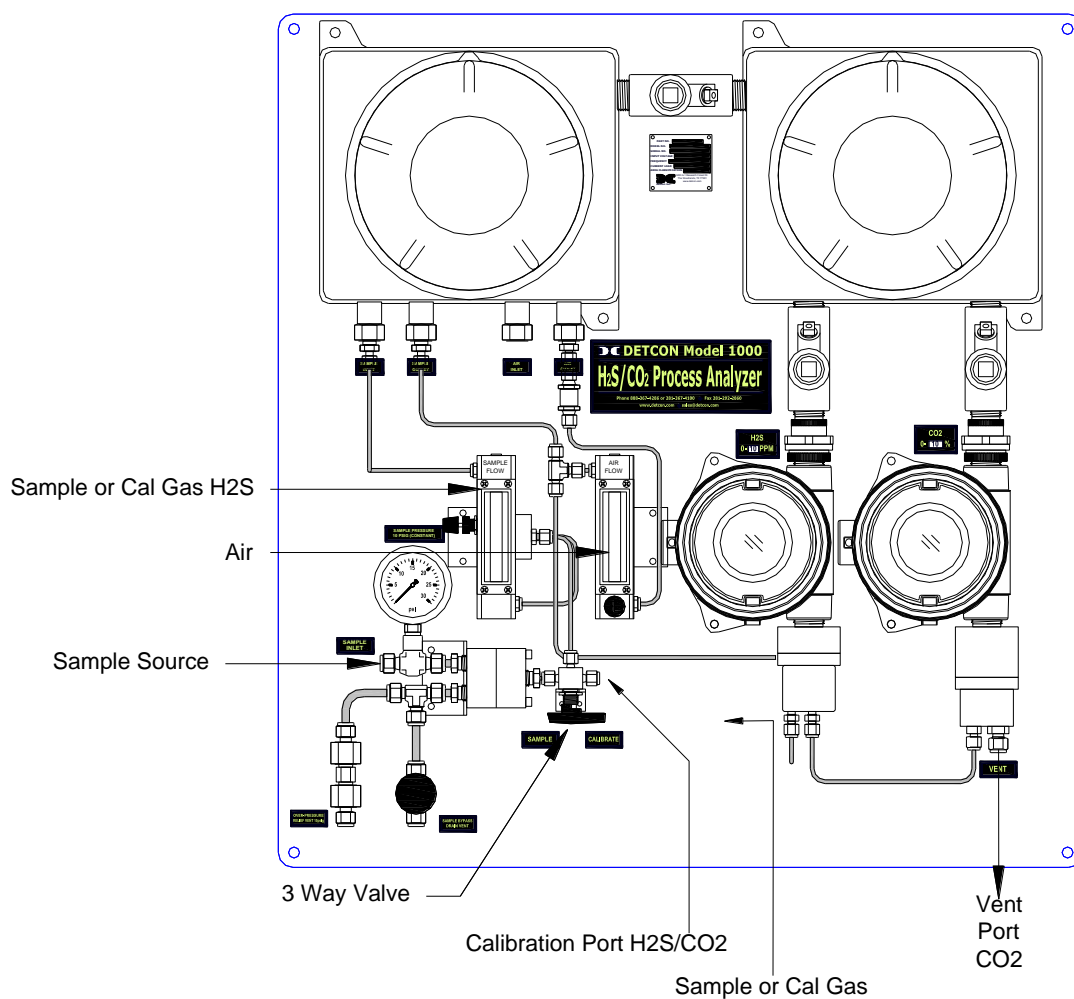
Figure 21 Rotameters and Gas Connections with Air Dilution
