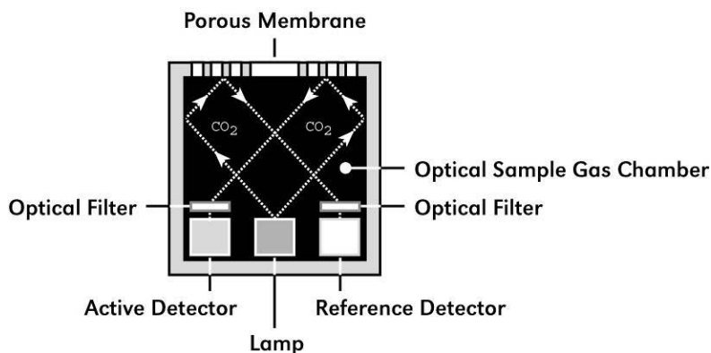
Figure 7 Sensor Diagram
