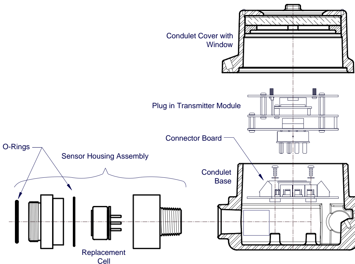
Figure 25 DM-624 Replacement Parts
