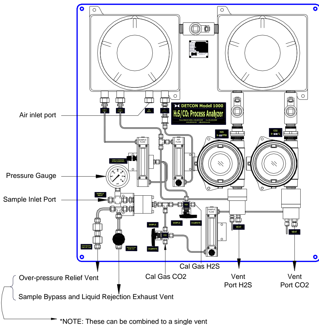
Figure 15 Port Identification
