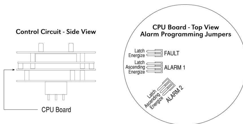
Figure 18 Alarm Jumpers
