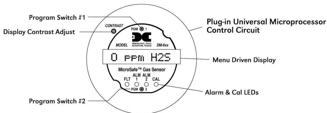
Figure 4 DM-624 Control Circuit
