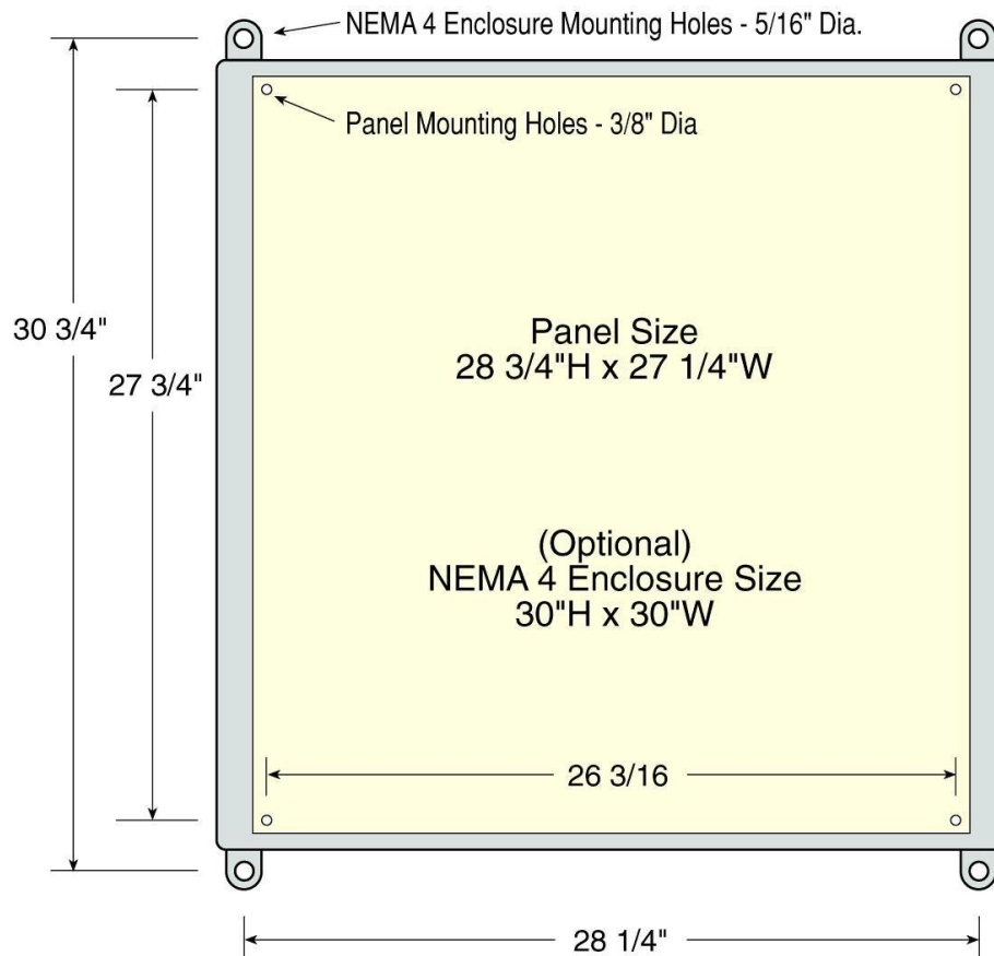
Figure 14 Unit Dimensions
