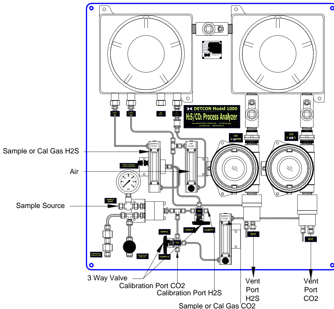
Figure 20 Rotameters and Gas Connections
