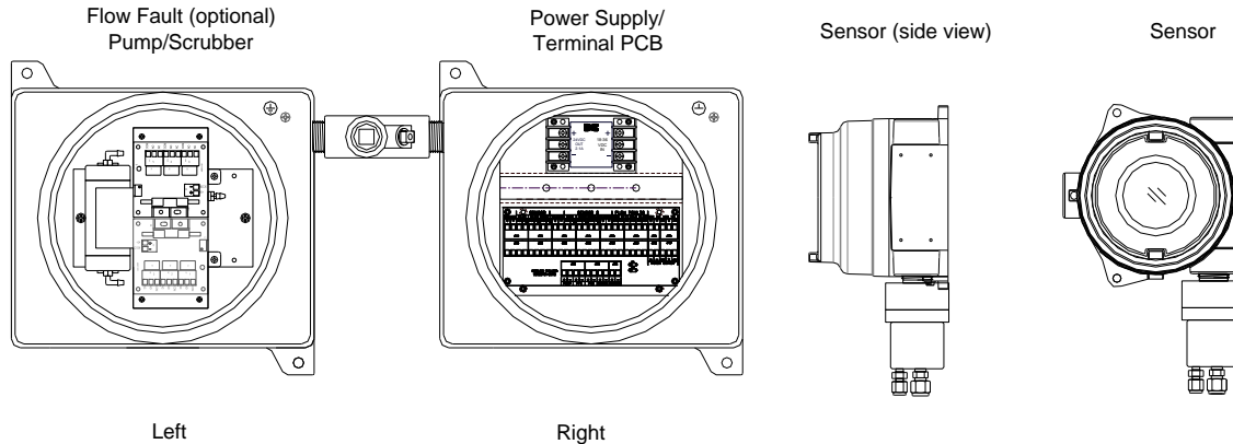
Figure 13 Enclosures
