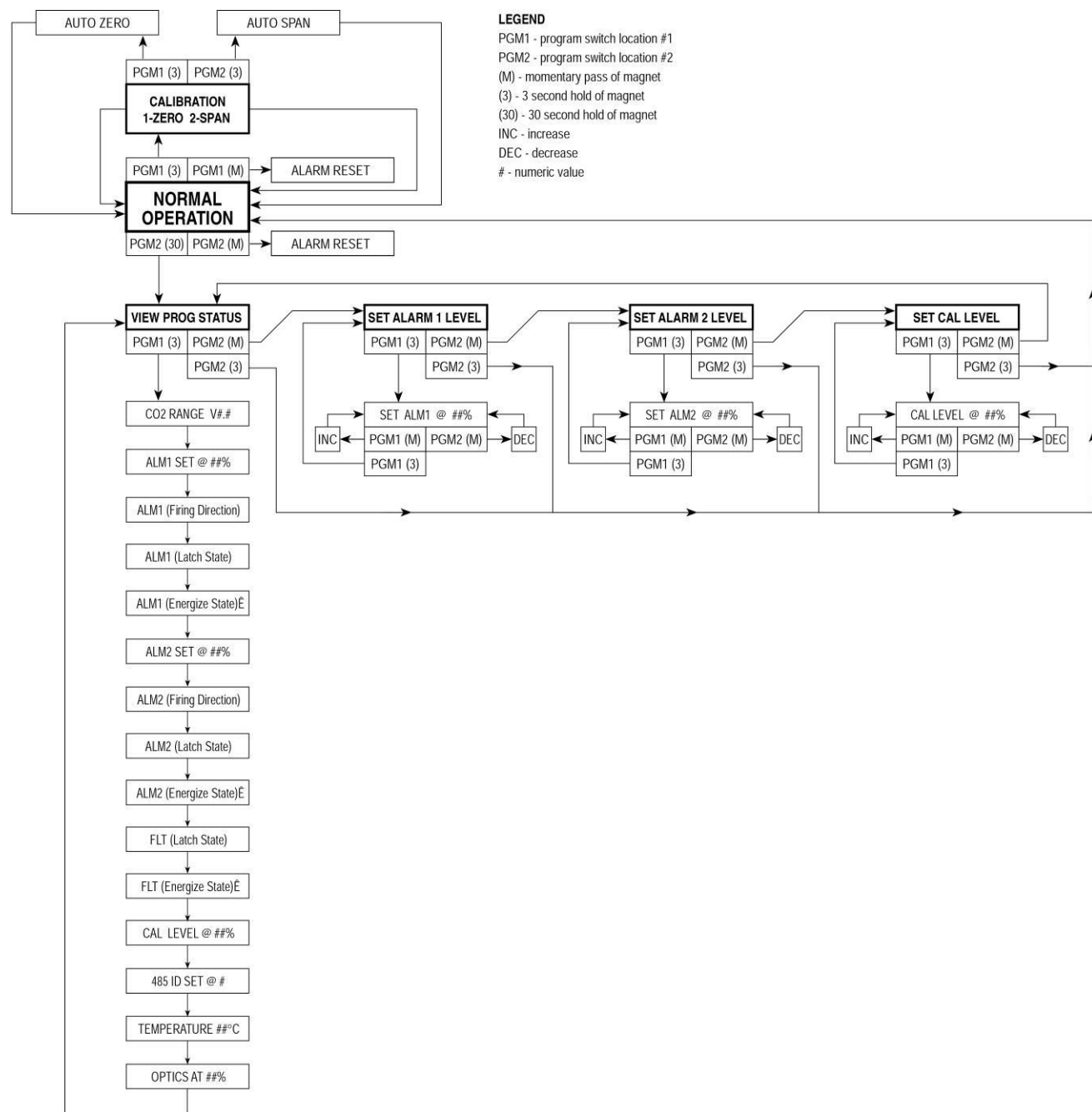
Figure 24 IR-640/IR/642 Software Flow Chart
