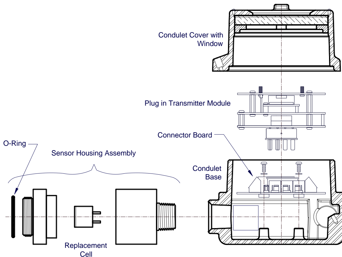
Figure 26 IR-640/IR-642 Replacement Parts
