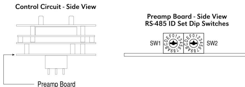
Figure 19 RS-485 Dip Switches
