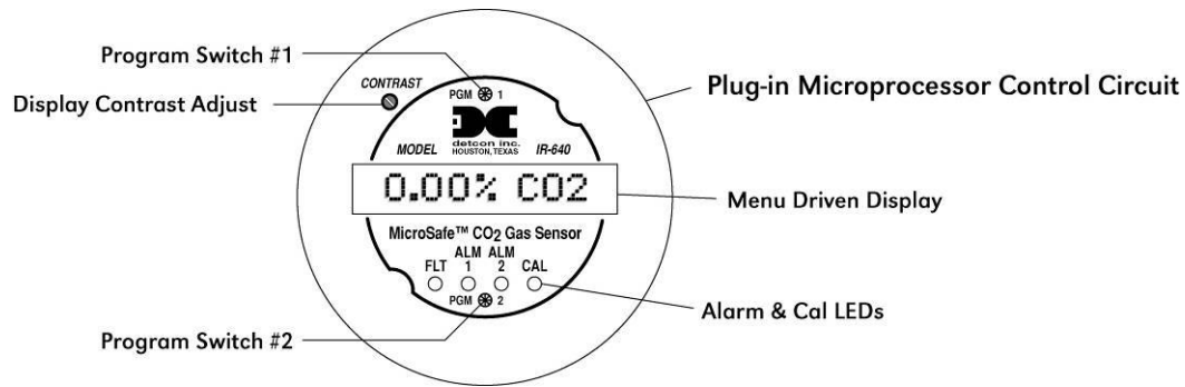
Figure 11 Control Circuit
