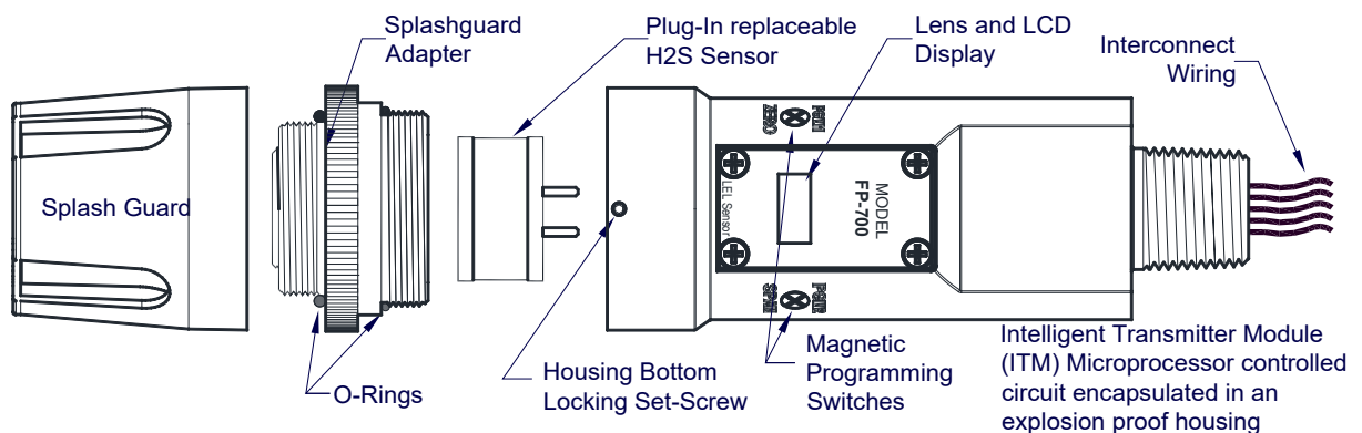
Figure 6 Sensor Assembly Breakaway
