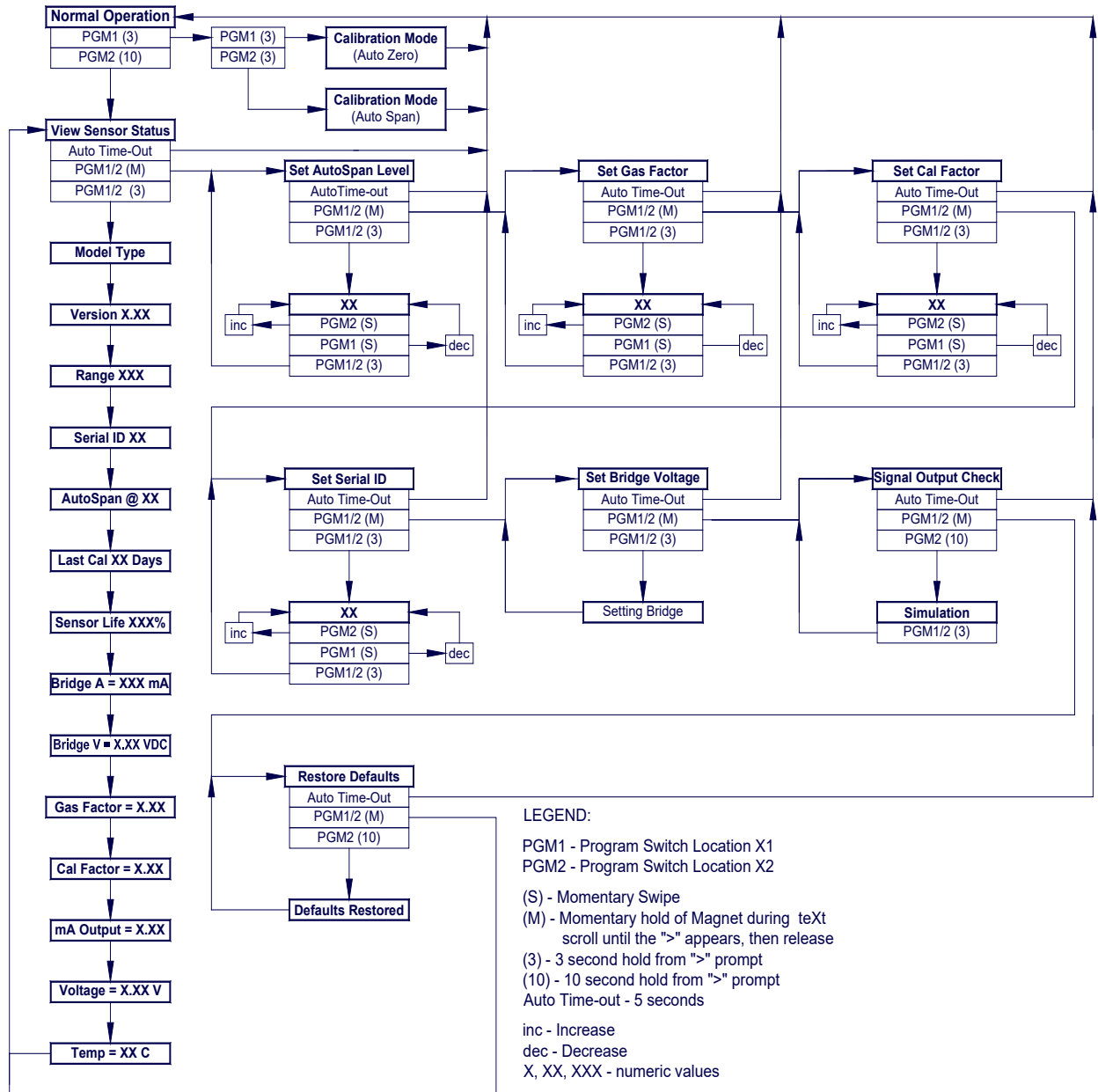
Figure 15 FP-700 Software Flowchart
