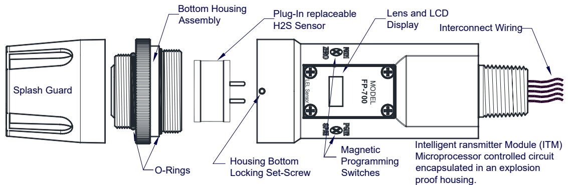
Figure 16 Sensor Assembly
