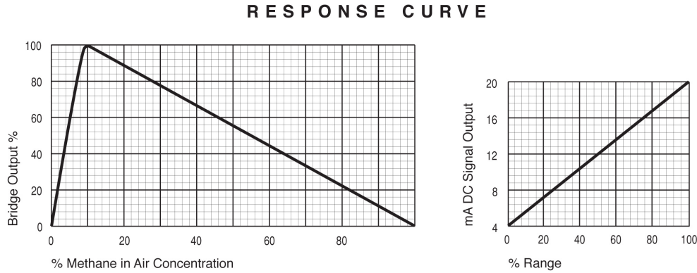
Figure 3 Response Curves
