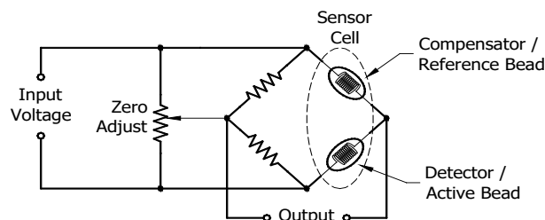
Figure 2 Wheatstone Bridge
