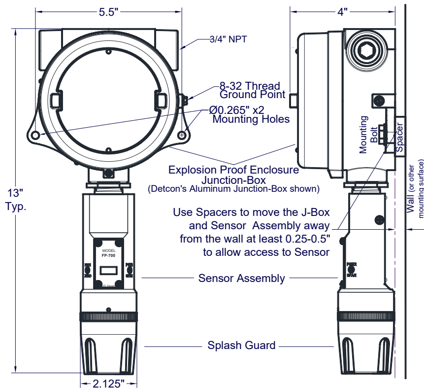
Figure 10 Outline and Mounting Dimensions (Aluminum Junction Box)
