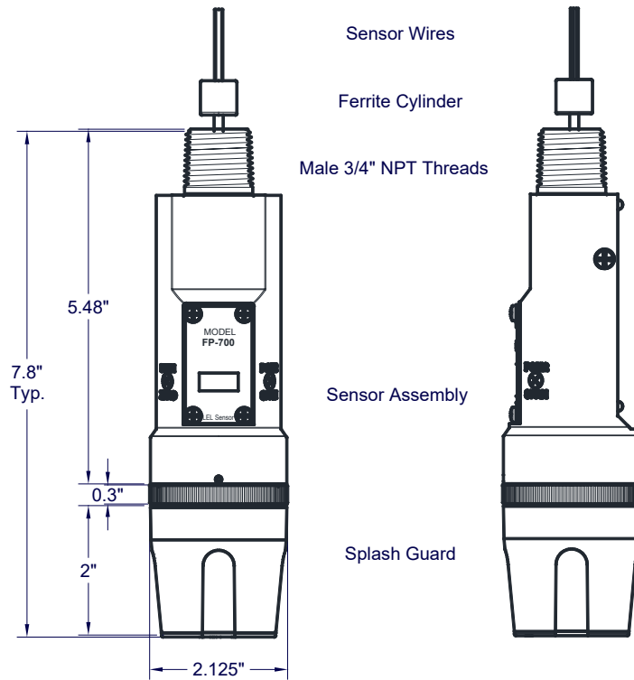
Figure 8 Outline and Mounting Dimensions (Sensor Assembly only)
