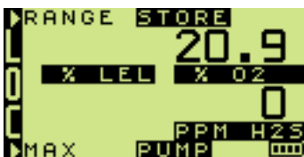
Fig. 3-31 Gas Present During Warm-up
