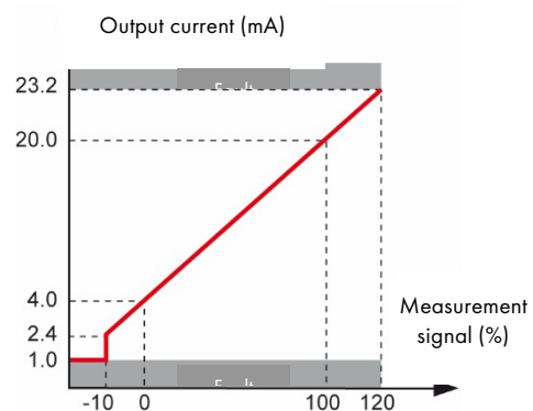
Figure 19: transfer curve for a 4-20 mA detector
