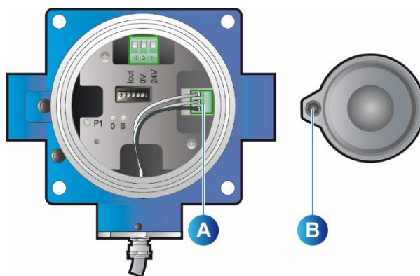
Figure 16 : OLCT 100 HT – elements specific to changing the high temperature sensor
