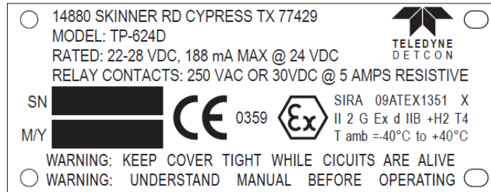
Figure 6 TP 624D ATEX Approval Label
