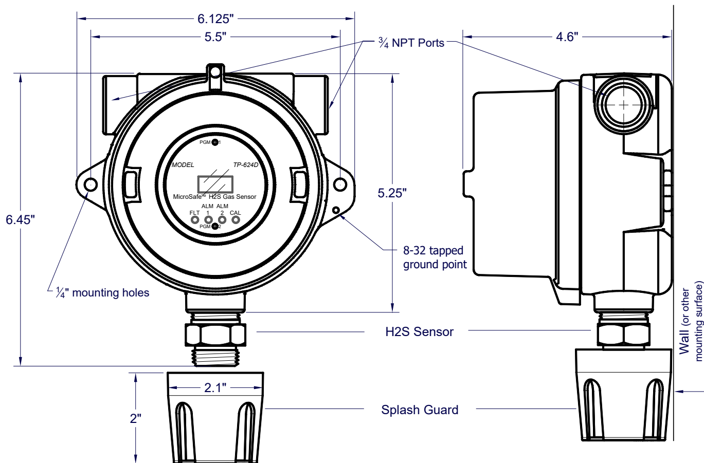
Figure 7 Typical Outline and Mounting Dimensions
