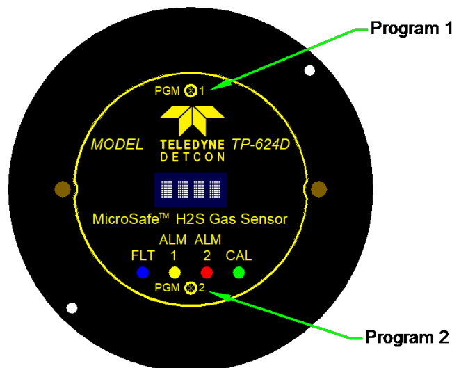
Figure 11 Magnetic Programming Switches
