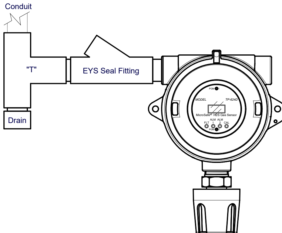
Figure 8 Typical Installation
