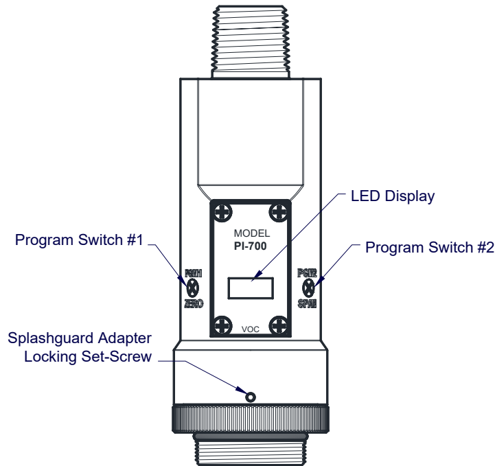
Figure 3 Sensor Assembly Front View
