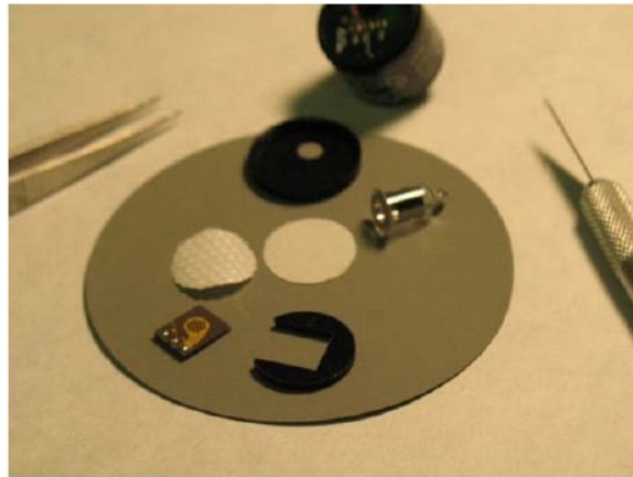
Figure 22 Lamp cleaning
