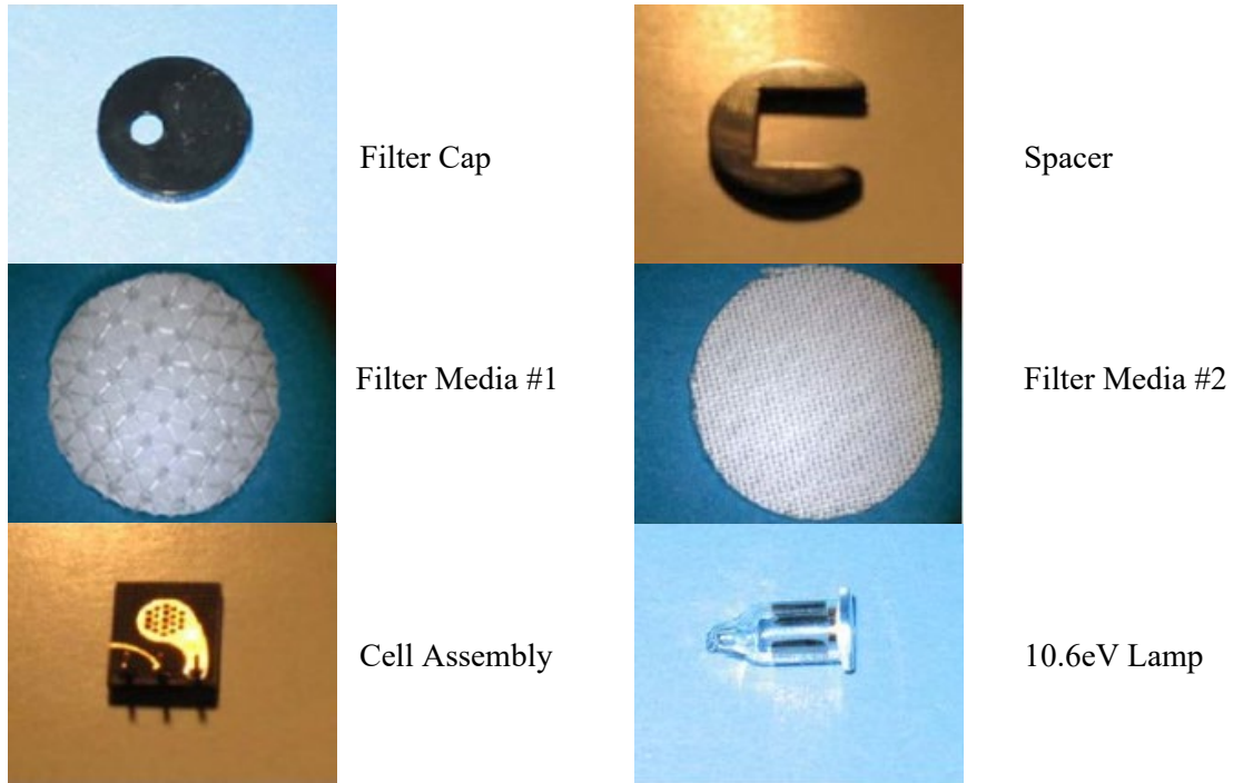
Figure 16 Sensor Cell Parts
