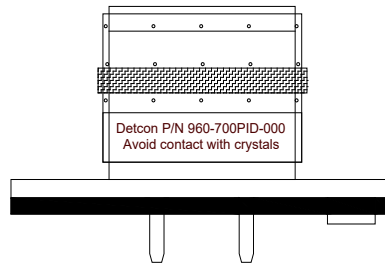
Figure 15 Plug-in sensor with Moisture control packet
