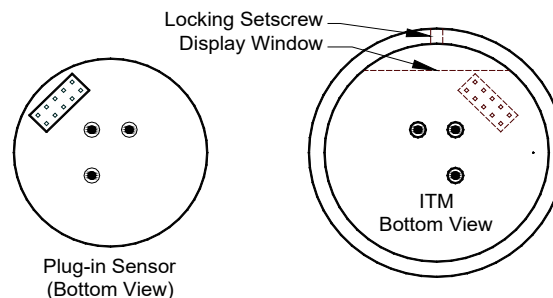
Figure 31 Sensor Cell and ITM Mating
