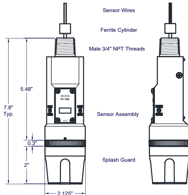
Figure 6 Outline and Mounting Dimensions (Sensor Assembly only)
