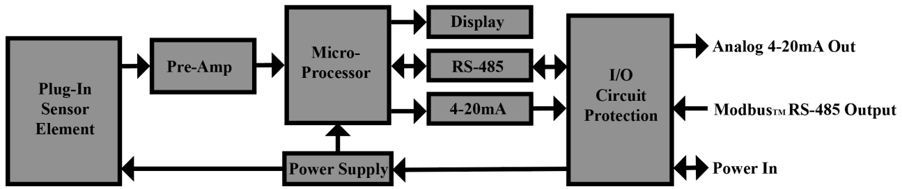
Figure 2 ITM Circuit Functional Block Diagram
