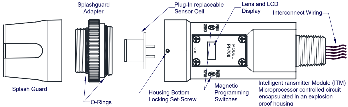
Figure 30 Sensor Assembly
