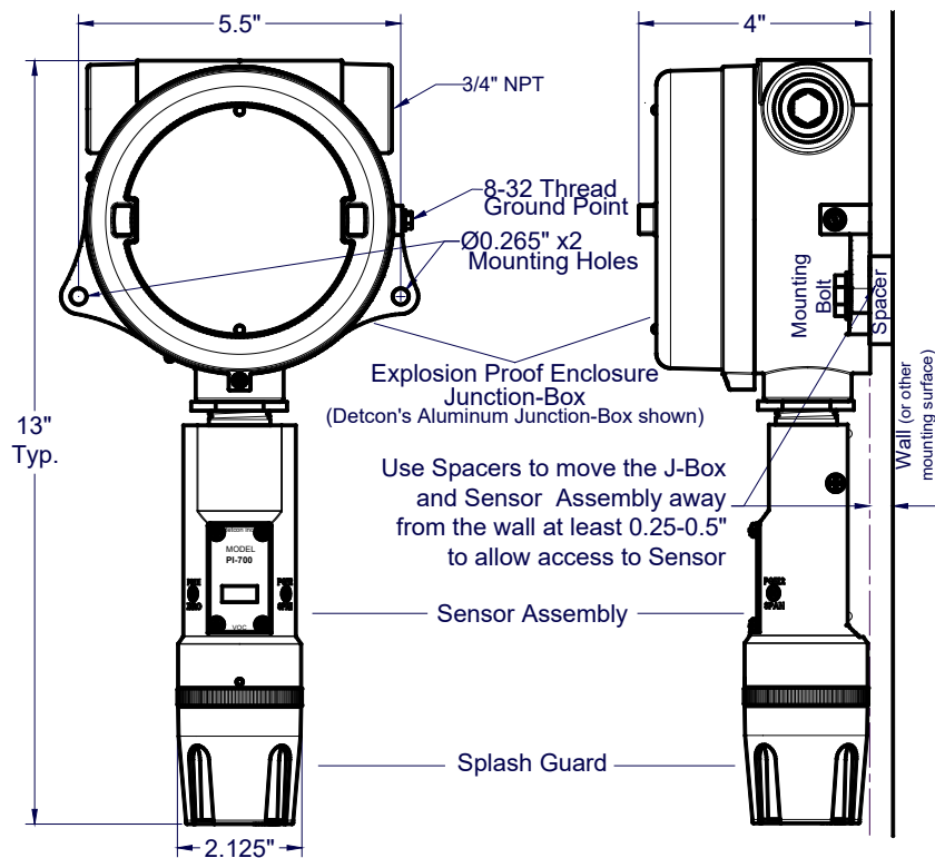
Figure 8 Outline and Mounting Dimensions (Aluminum Junction Box)
