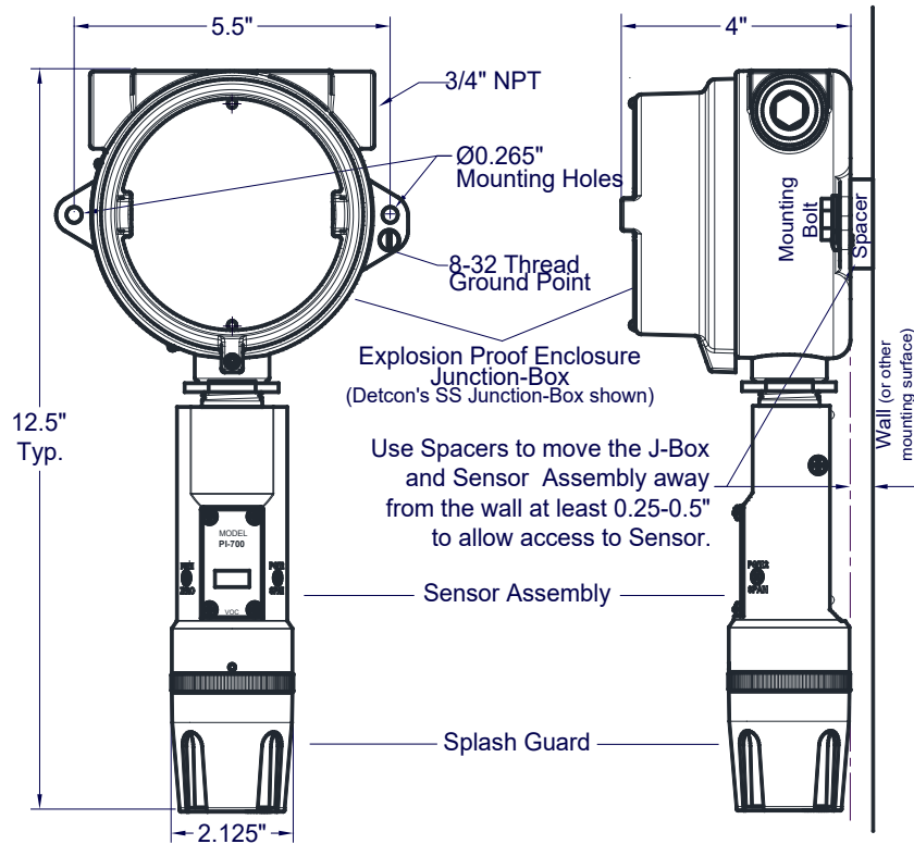
Figure 7 Outline and Mounting Dimensions (Stainless Steel Junction Box)
