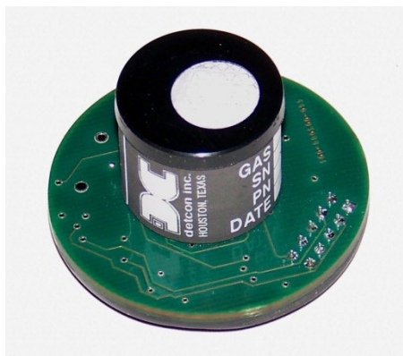
Figure 5 Intelligent Plug-in Sensor Assembly Breakaway
