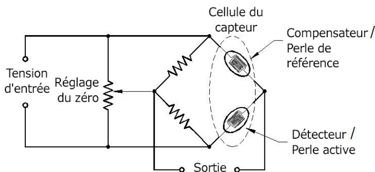
Figure 2 : Pont de Wheatstone
