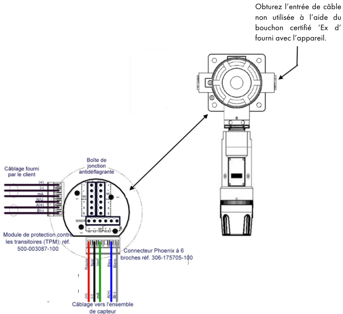
Figure 10 : Installation standard
