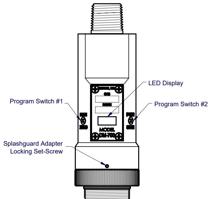
Figure 13 Magnetic Programming Switches
