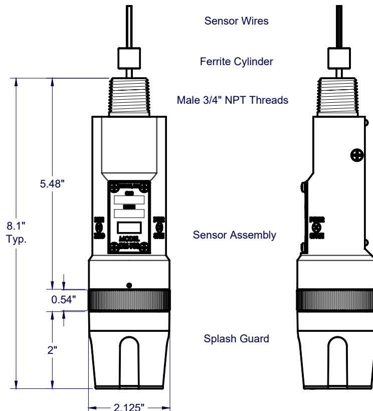
Figure 7 Outline and Mounting Dimensions (Sensor Assembly Only)
