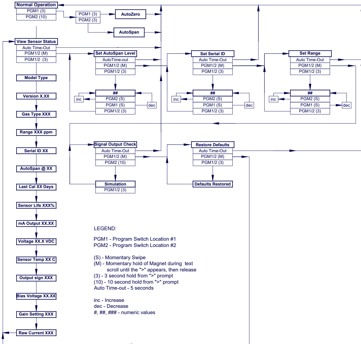
Figure 14 DM-700 Software Flowchart
