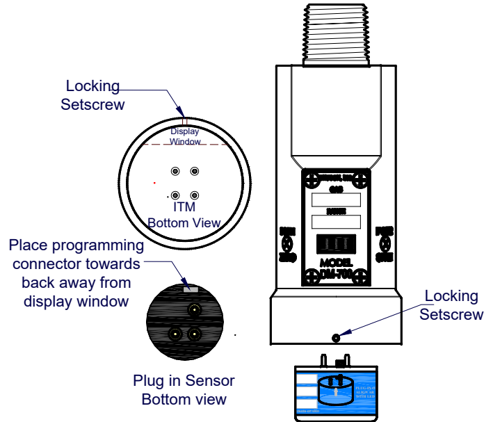
Figure 17 Sensor Cell and ITM Mating
