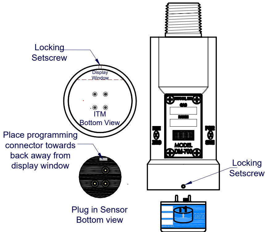
Figure 16 Sensor Cell and ITM Mating
