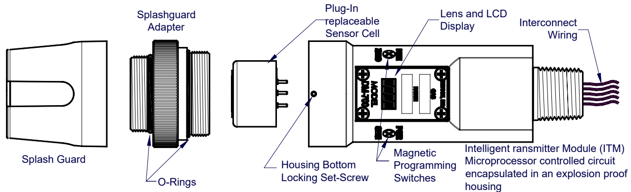
Figure 15 Sensor Assembly
