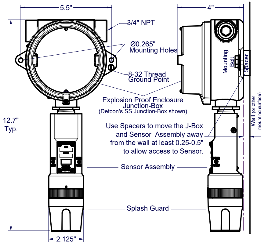
Figure 8 Outline and Mounting Dimensions (Stainless Steel Junction Box)
