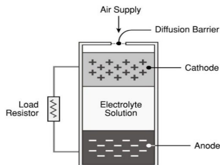
Figure 2 Construction of Galvanic Cell
