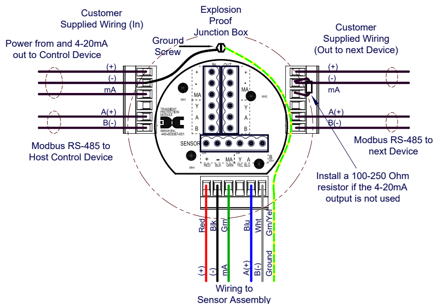
Figure 11 Sensor Wire Connections
