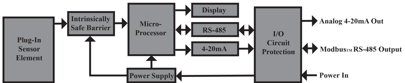
Figure 3 ITM Circuit Functional Block Diagram
