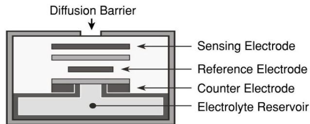
Figure 1 Construction of Electrochemical Toxic Sensor
