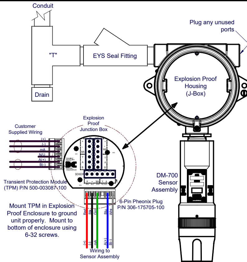
Figure 10 Typical Installation
