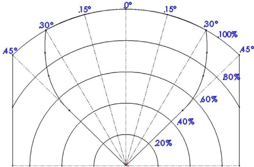
Figure 11 : - Horizontal field of view
