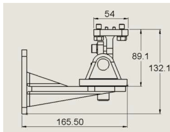
Figure 14 : Tilt mount base – Side View
