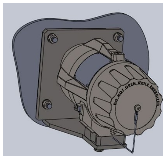
Figure 9 : Duct Mount SP-F- DMX-S02
