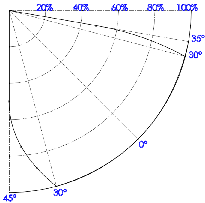
Figure 12 : Vertical field of view
