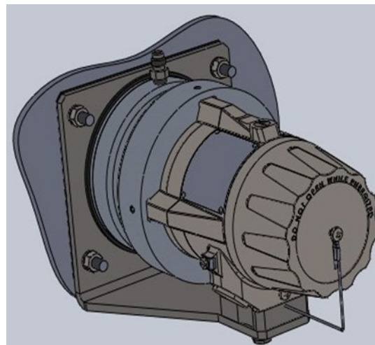
Figure 9 : Duct Mount SP-F- DMX-S02
