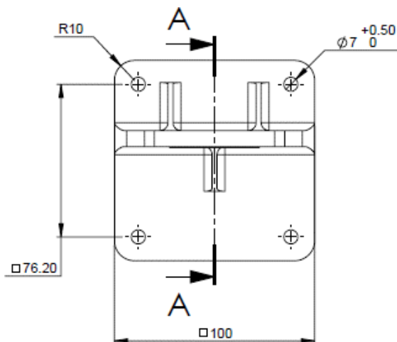
Figure 13 : Tilt Mount Base - Plate View
